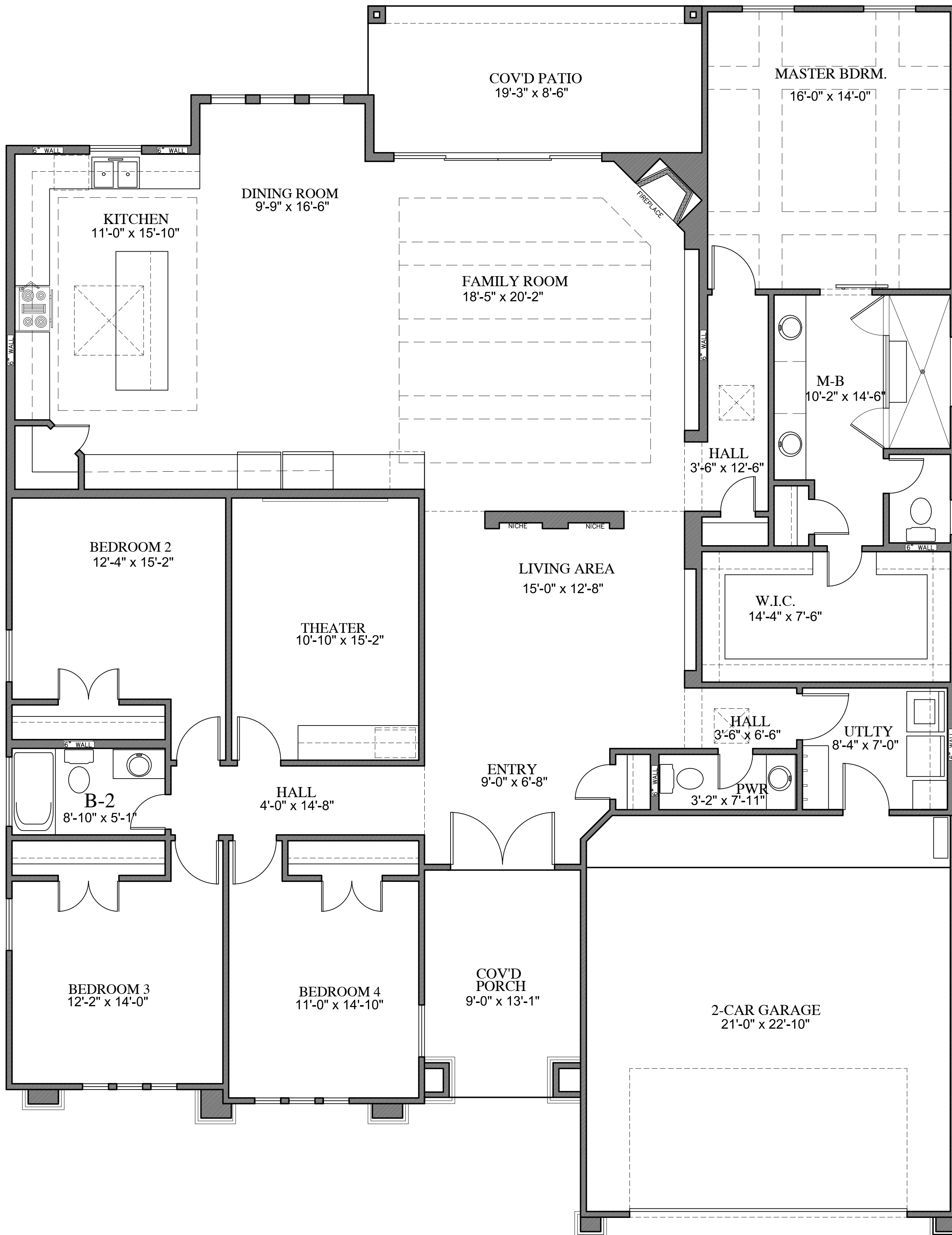
FLOOR PLAN
