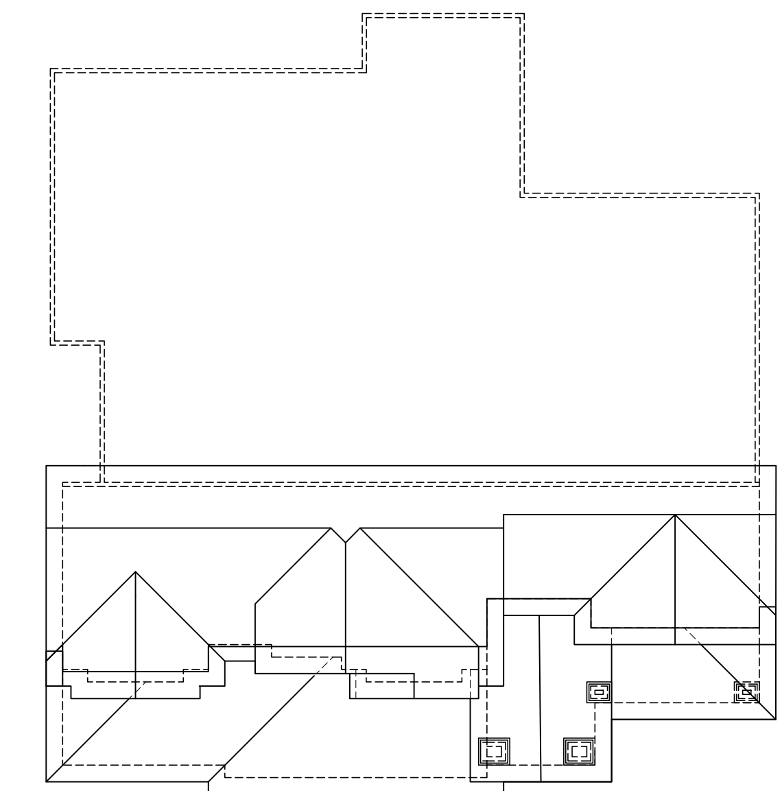
PRELIMINARY ROOF LAYOUT
