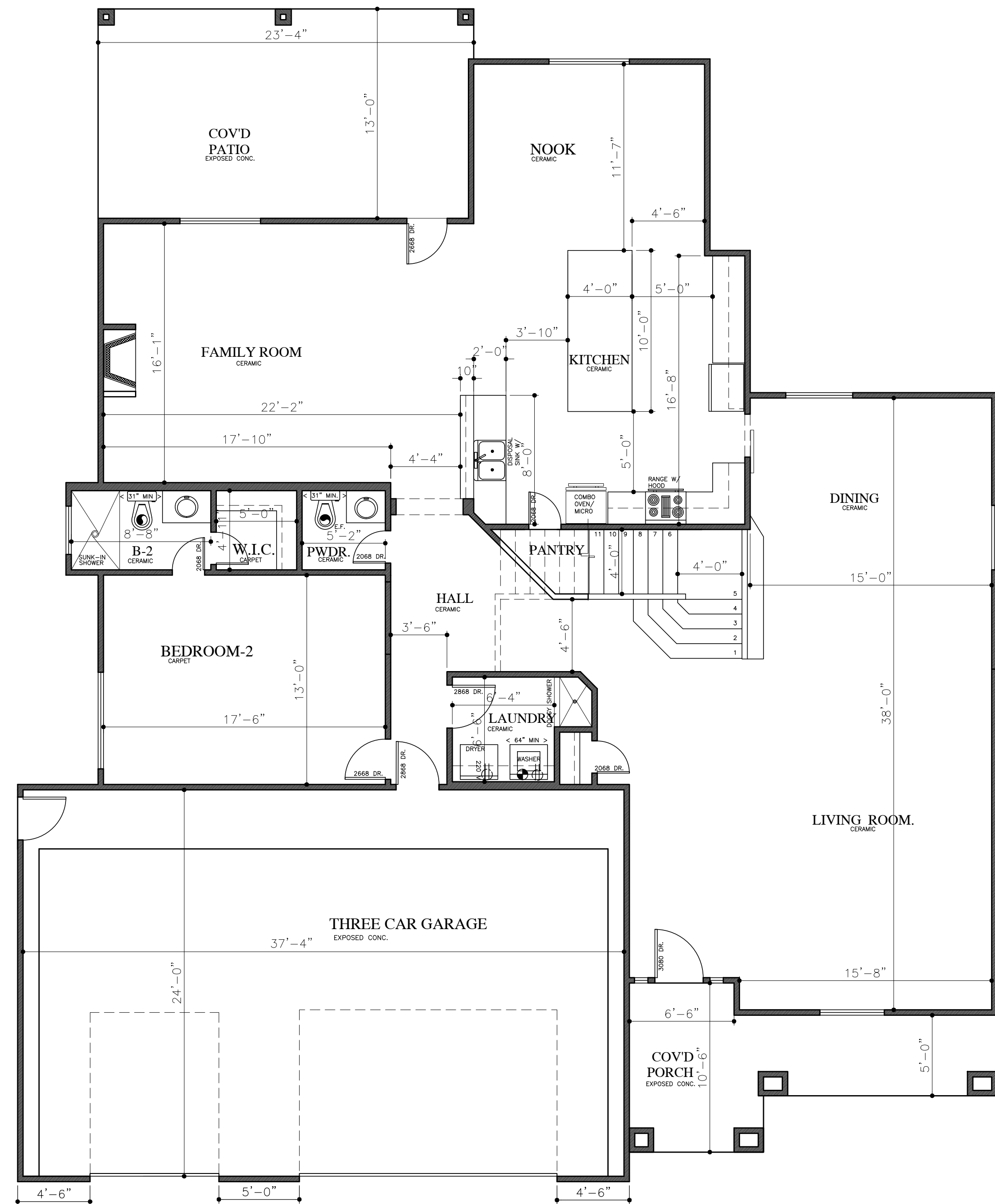
1ST. FLOOR PLAN
