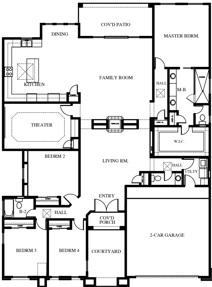
FLOOR PLAN SCALE: NTS
