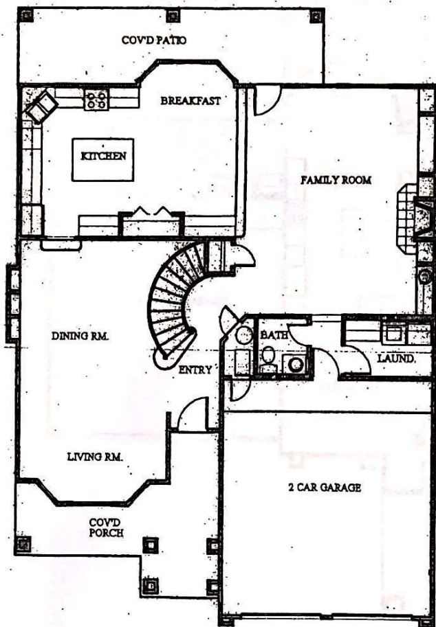
FIRST FLOOR SCALE 1/4" = 1'-0"
