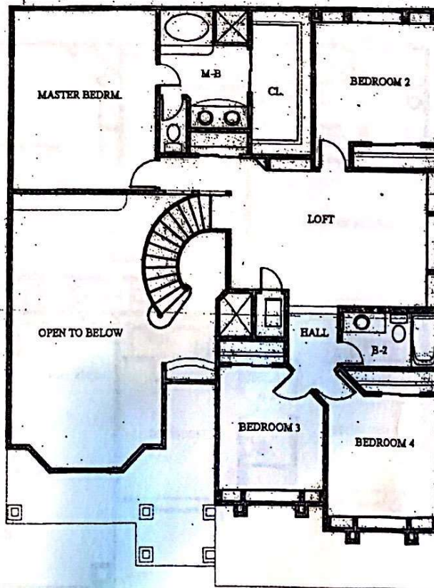
SECOND FLOOR SCALE 1/4" = 1'-0"
