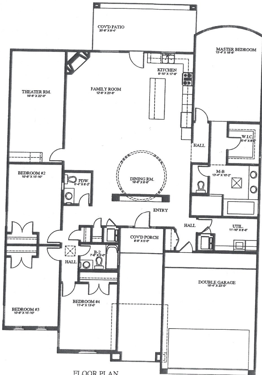
FLOOR PLAN SCALE: NS
